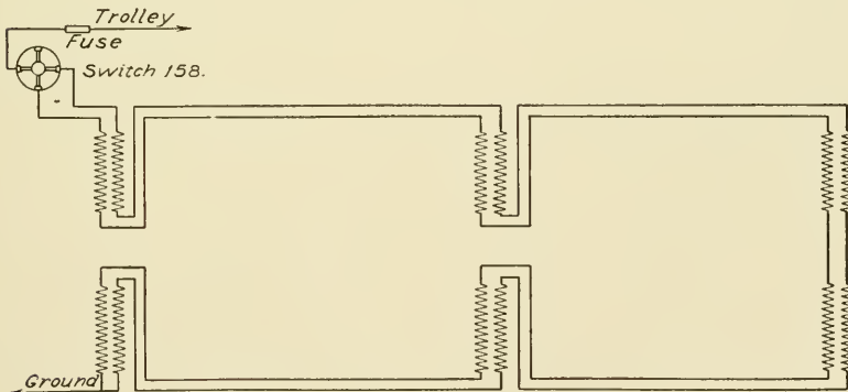
Fig. 112. Diagram of Car Heater Circuits
